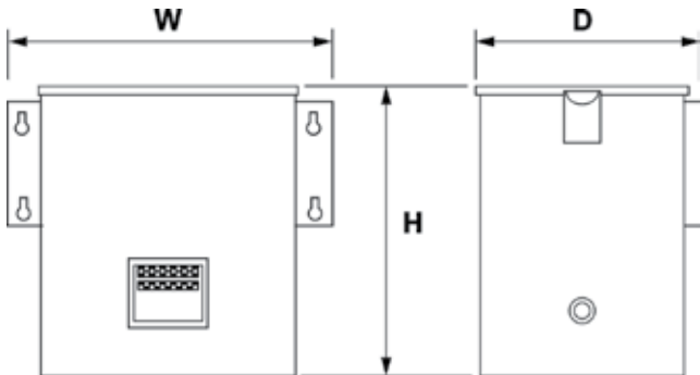
Style 4 - Encapsulated
